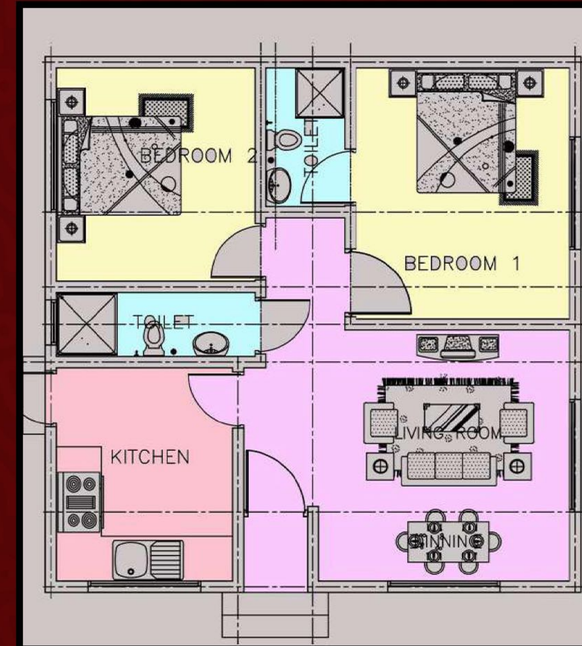
SALLY 'S FLOOR PLAN
