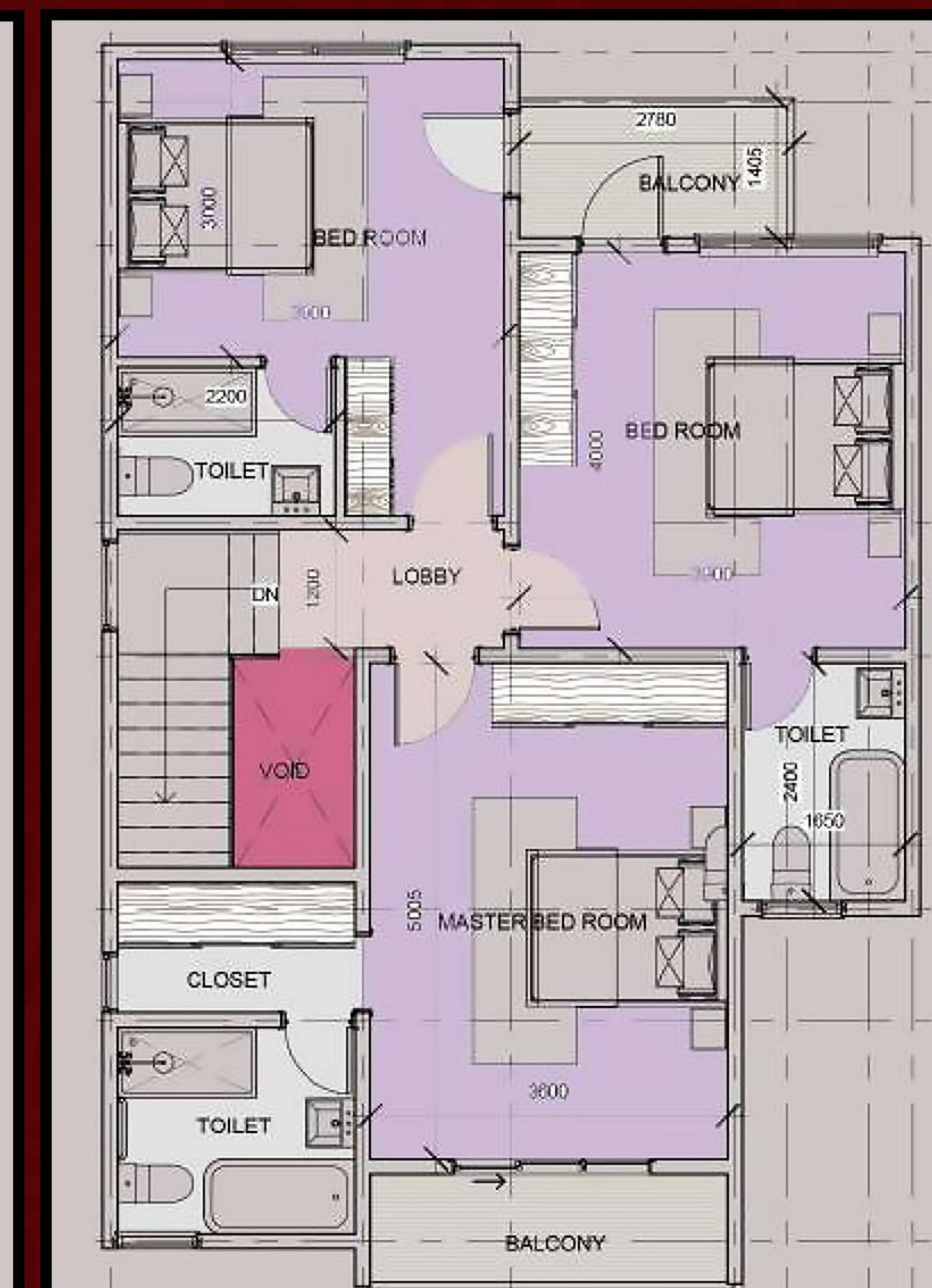
TOP FLOOR
